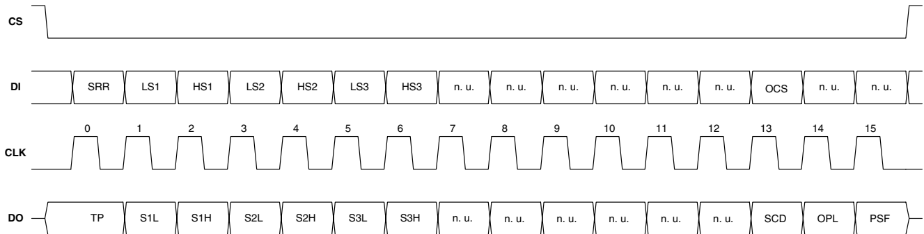
Figure 3-1. Data Transfer
